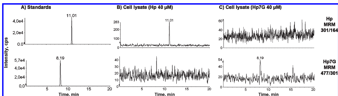
Figure 2. MRM trace chromatograms at hesperetin (301/164) and hesperetin-7-O-glucuronide (477/301) transitions from (A) standards; (B) cell lysate after 24 h of exposure to 40 \mu M Hp; and (C) cell lysate after 24 h of exposure to 40 \mu M Hp7G.
